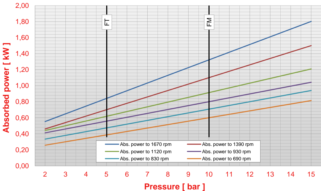
Pump F FT FM 40 pressure - abs. power chart (viscosity 50 cps)
