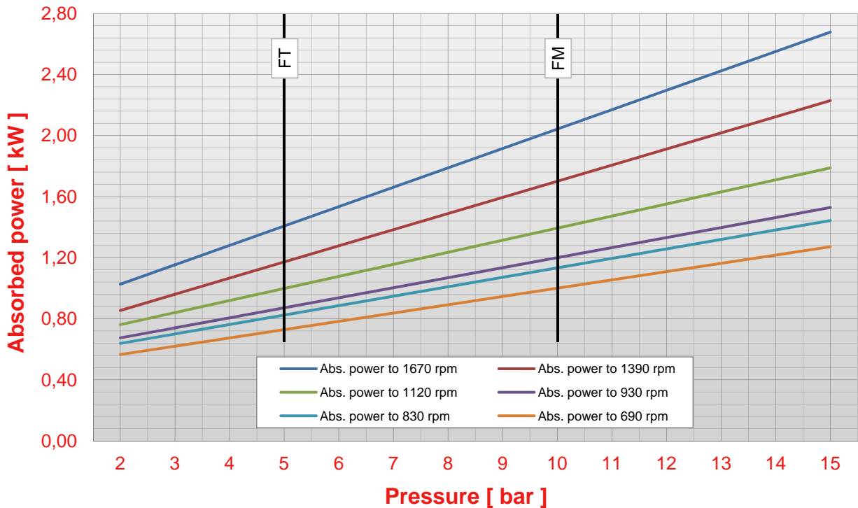
Pump F FT FM 70 pressure - abs. power chart (viscosity 50 cps)
