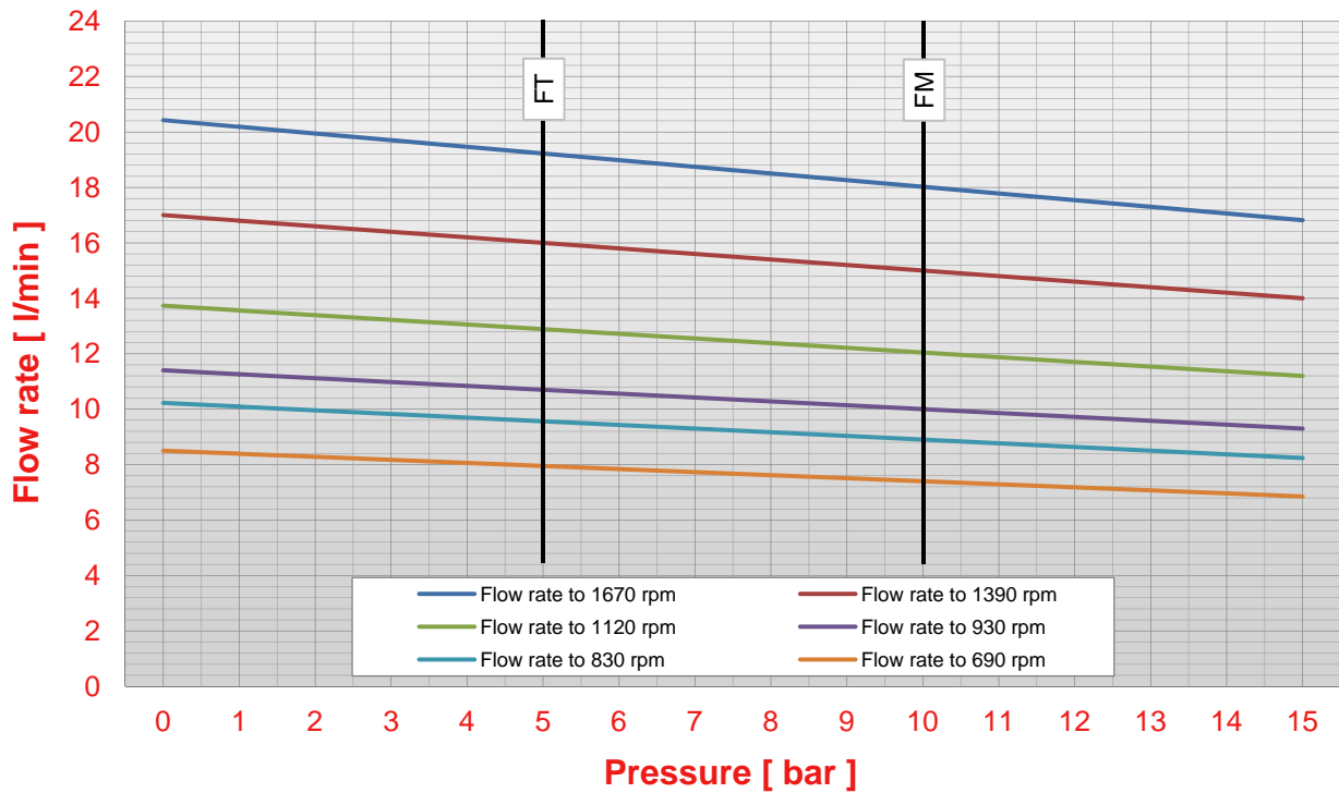
Pump F FT FM 15 pressure - flow rate chart (viscosity 50 cps)
