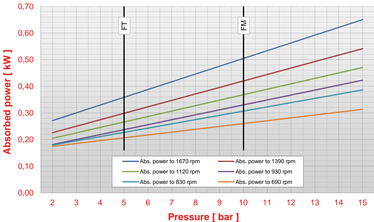
Pump F FT FM 15 pressure - abs. power chart (viscosity 50 cps)
