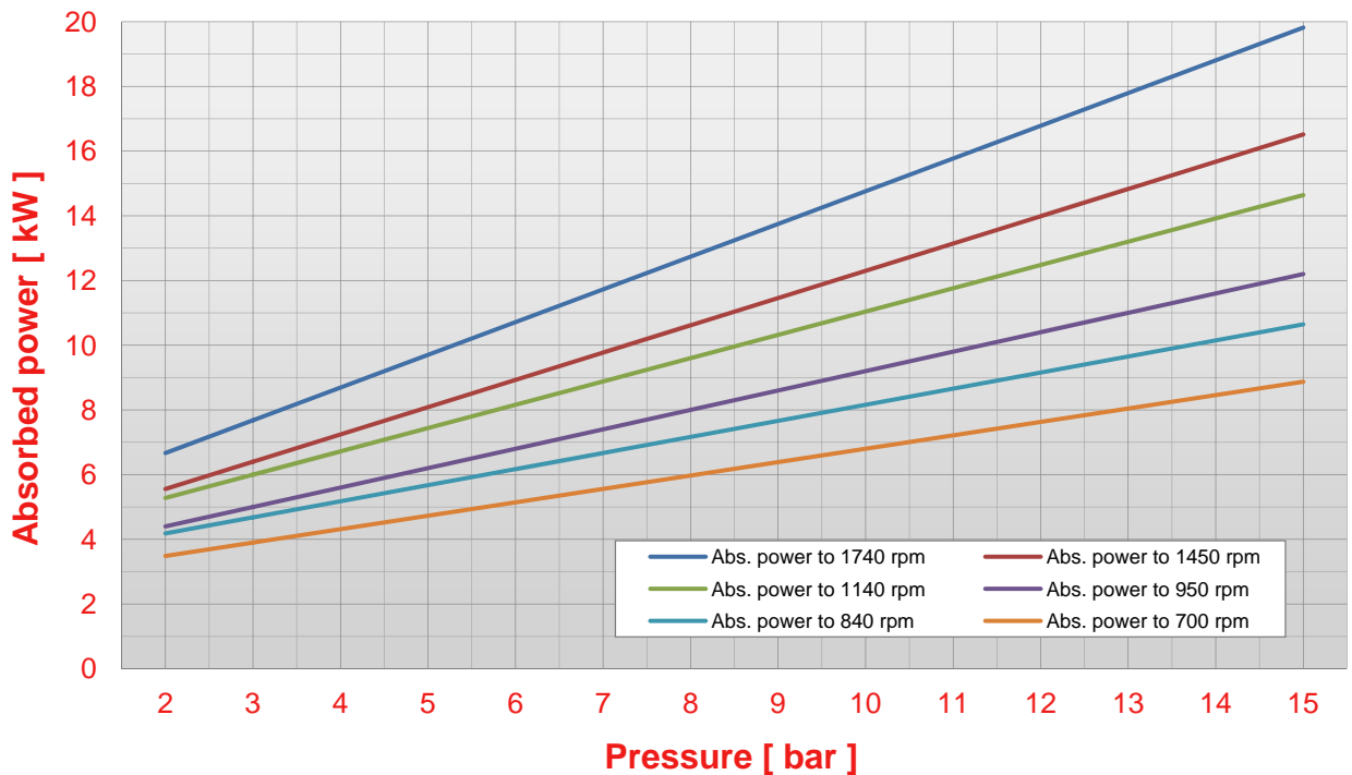
Pump S 500 pressure - abs. power chart (viscosity 50 cps)
