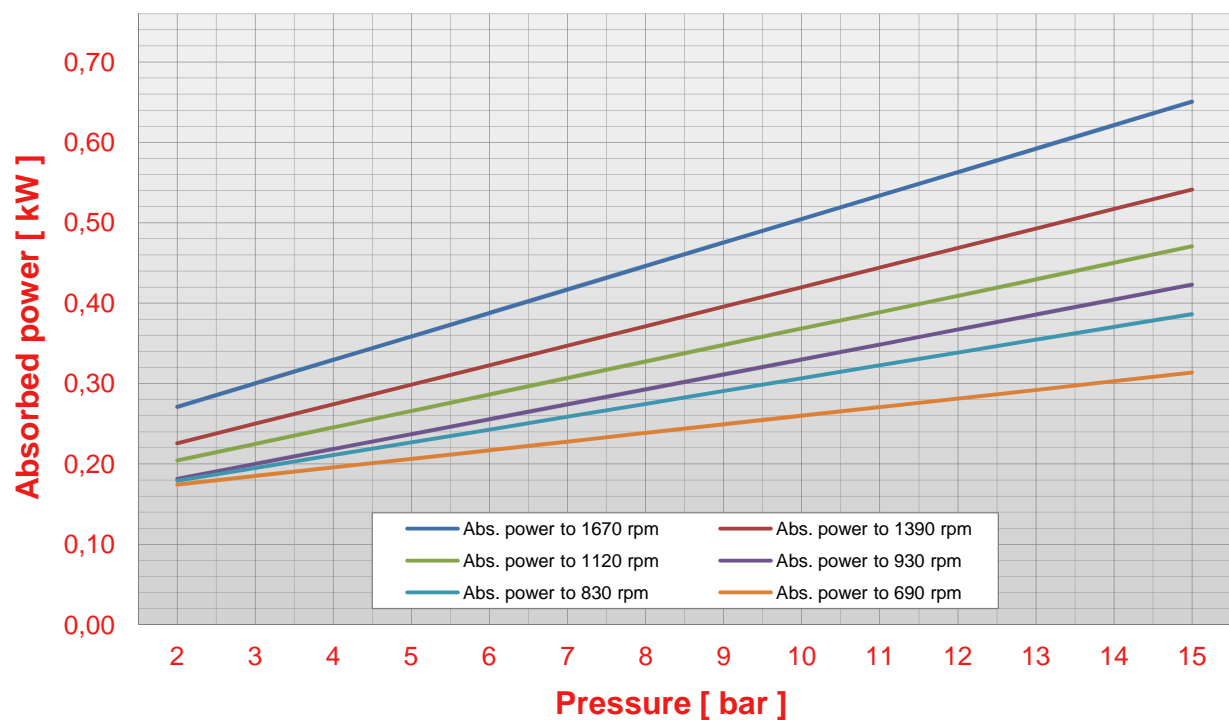
Pump SK 15 pressure - abs. power chart (viscosity 50 cps)
