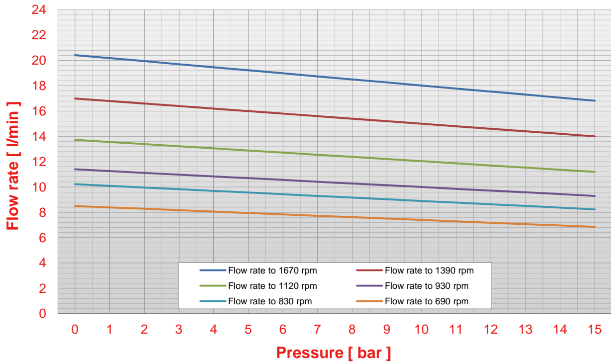
Pump SK 15 pressure - flow rate chart (viscosity 50 cps)
