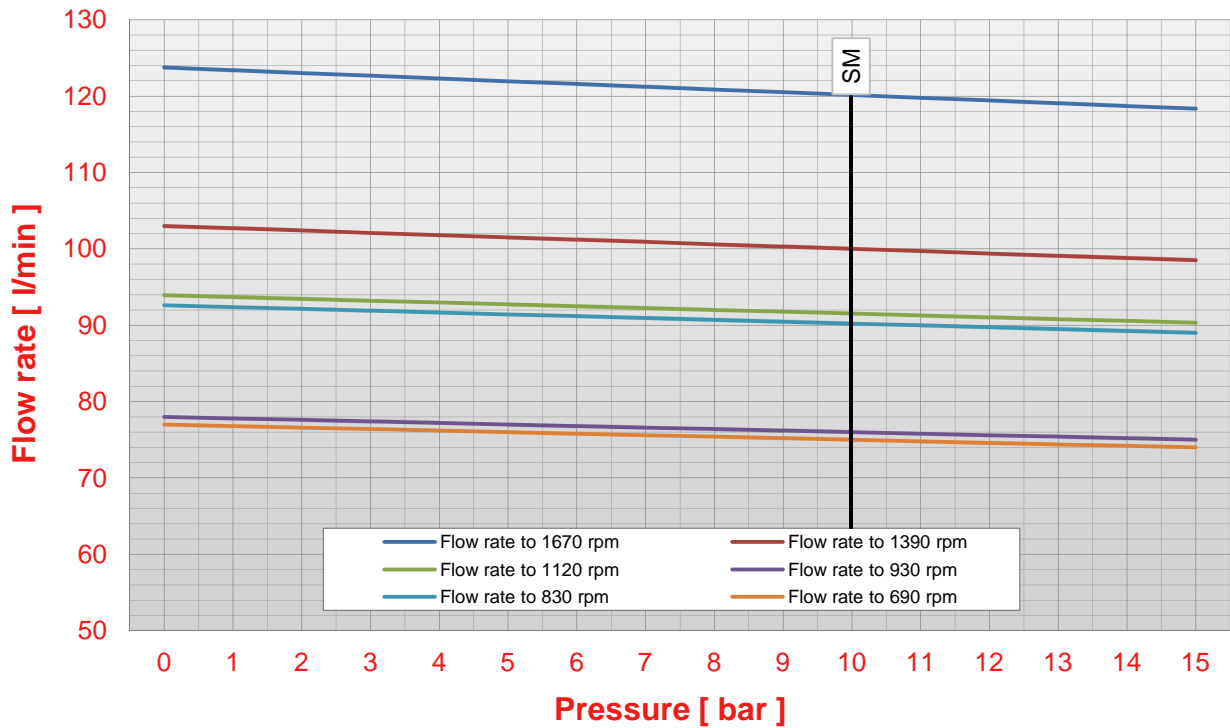
Pump S 100 pressure - flow rate chart (viscosity 50 cps)
