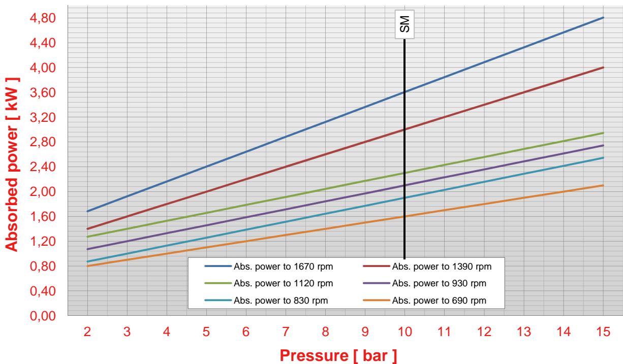
Pump S 100 pressure - abs. power chart (viscosity 50 cps)
