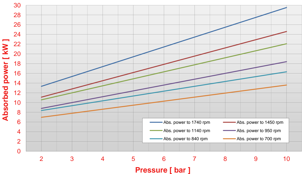
Pump S M00 pressure - abs. power chart (viscosity 50 cps)
