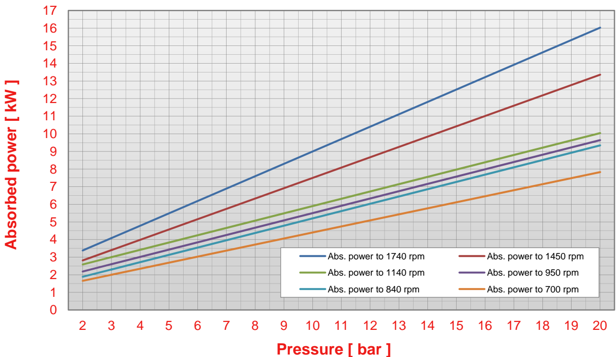
Pump S 320 pressure - abs. power chart (viscosity 50 cps)
