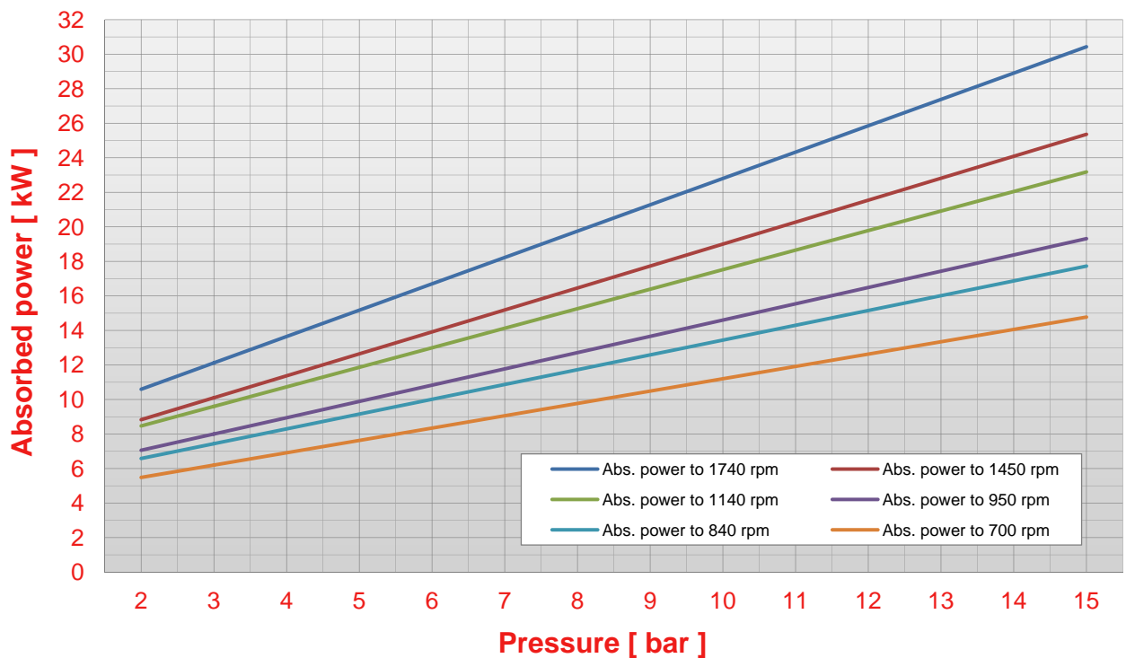
Pump S 800 pressure - abs. power chart (viscosity 50 cps)
